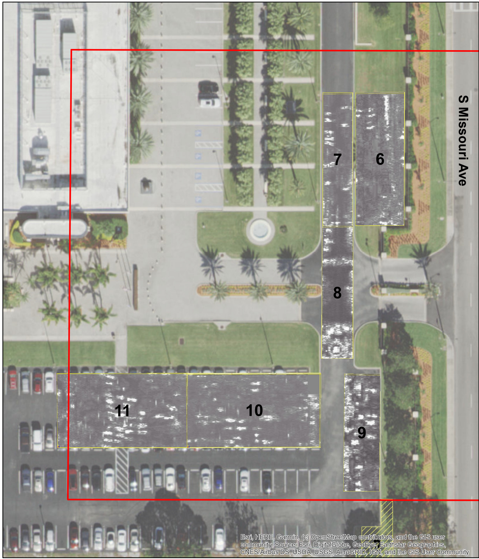
Figure 2: Overview of GPR results for grids 6 - 11. Results shown are from between 75-125 cm below ground surface. GPR grid number is marked on each survey area.
