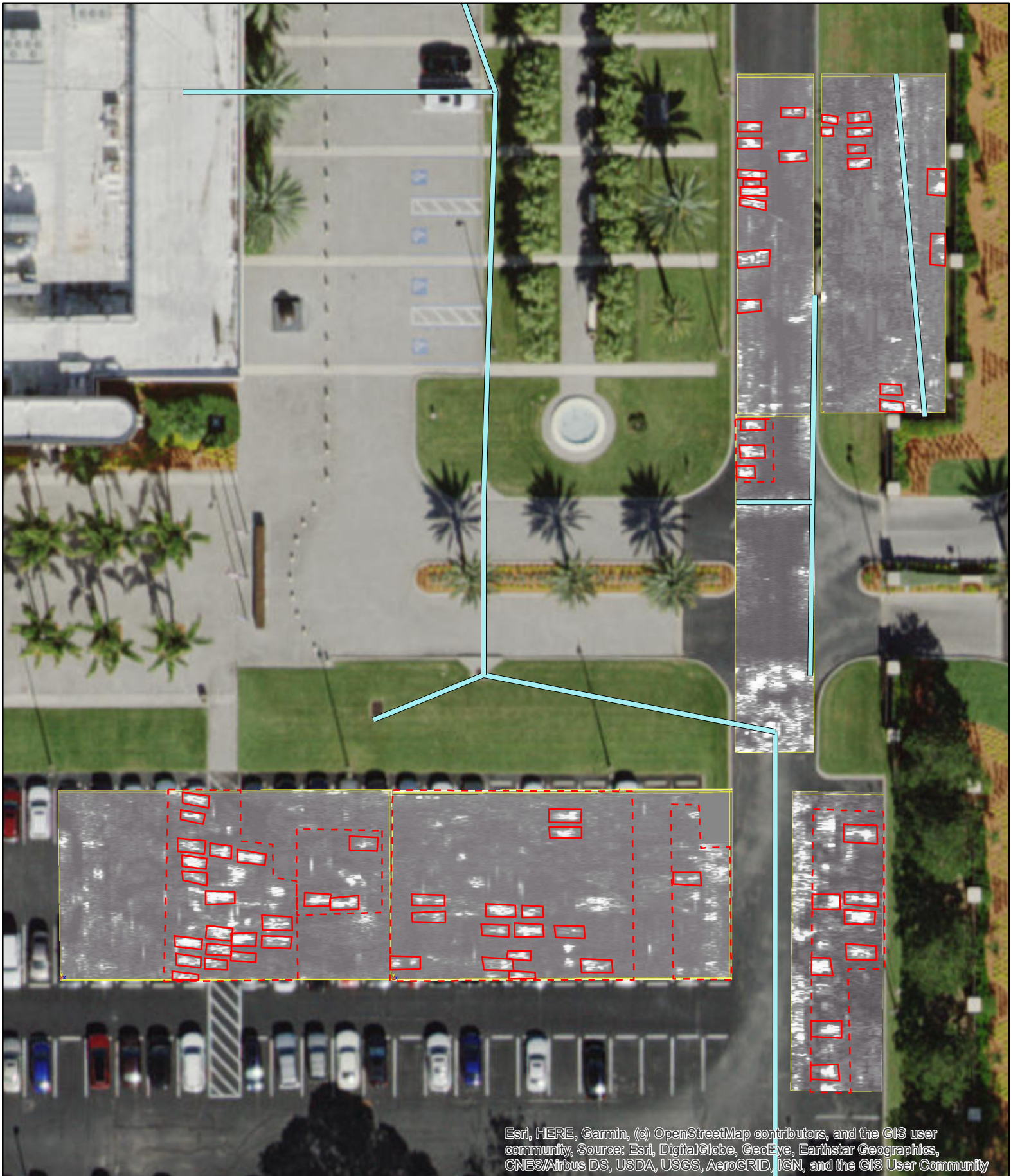
Figure 3: GPR results for grids 6-11. Areas marked in solid red are possible burials. Areas marked with a dashed red line are general areas of buried objects that could contain burials. Blue lines are buried utilities or trenches.
