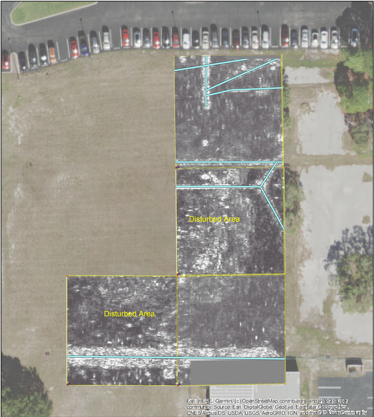
Figure 4: GPR results at 110 cm below surface with utility lines marked in blue.
