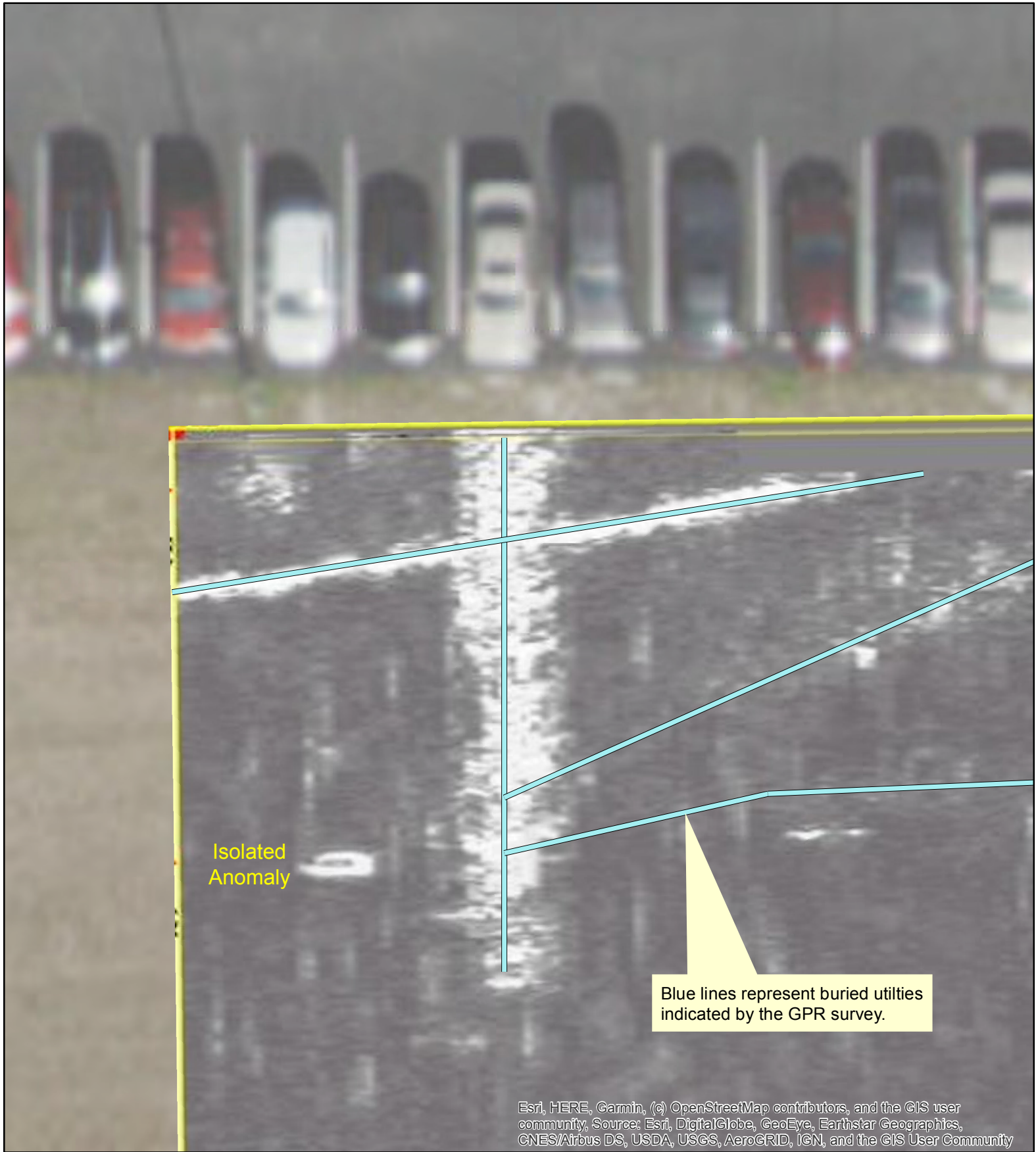
Figure 5: Isolated anomaly at around 150 cm below surface with surrounding utilities marked in blue.
